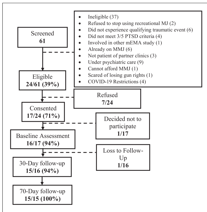
Fig. 1. Participant recruitment flowchart.
